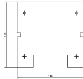
PCB MAX SIZE
