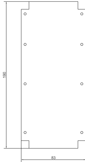
MAXIMUM PCB SIZE
